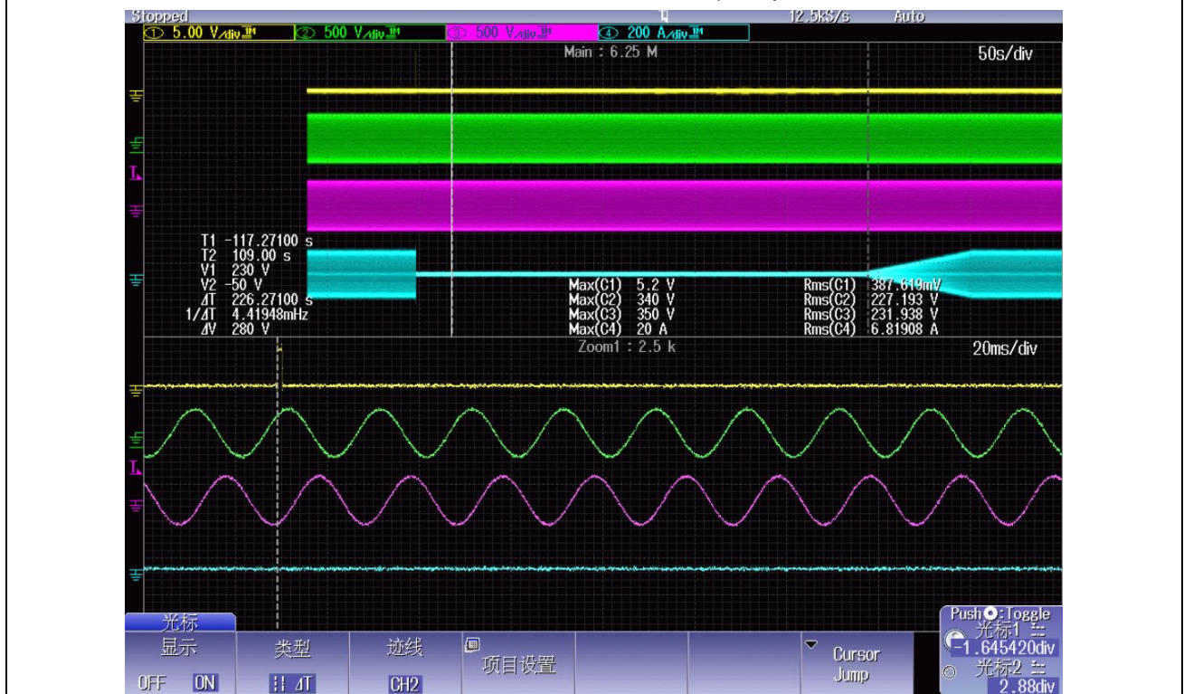
Reconnection after Over Frequency
