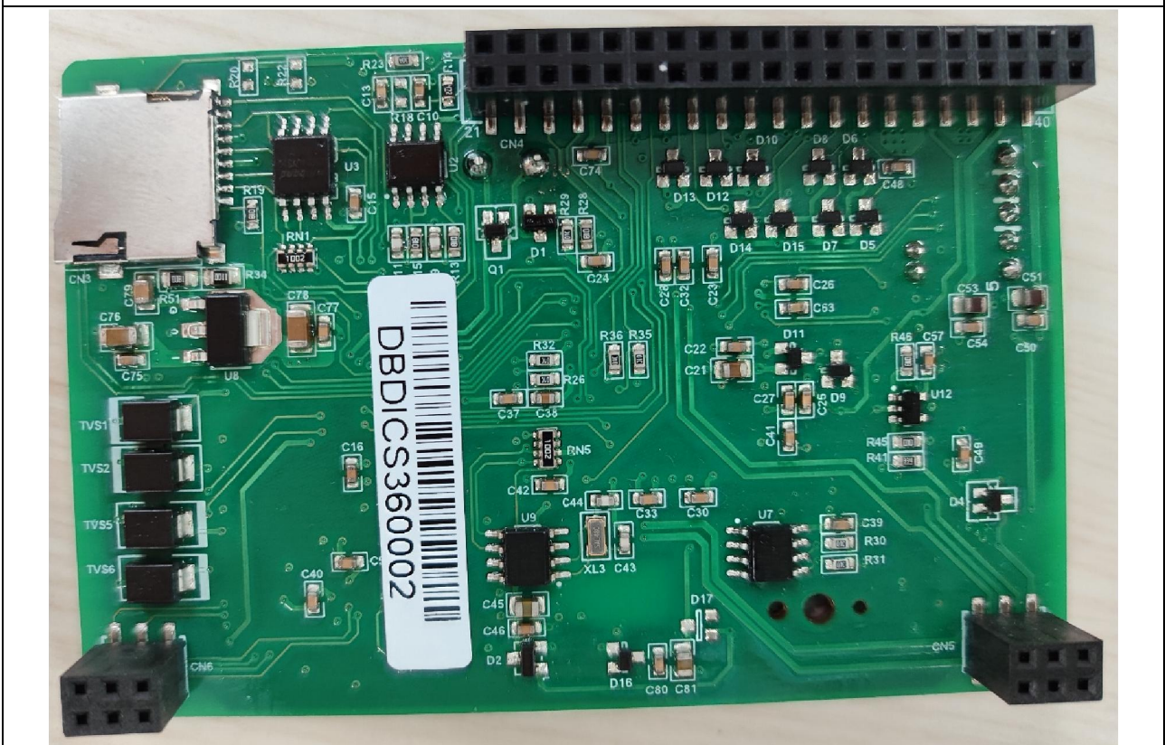
Bottom view of AC Charging Core Board, V 1.40
