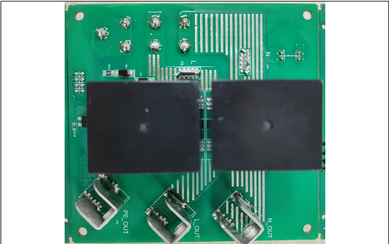
Top view of Single Phase AC Charging Connect Board, V 1.80
