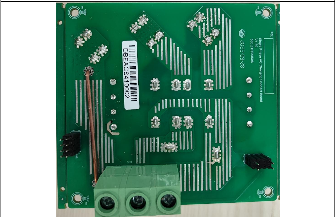
Bottom view of Single Phase AC Charging Connect Board, V 1.80
