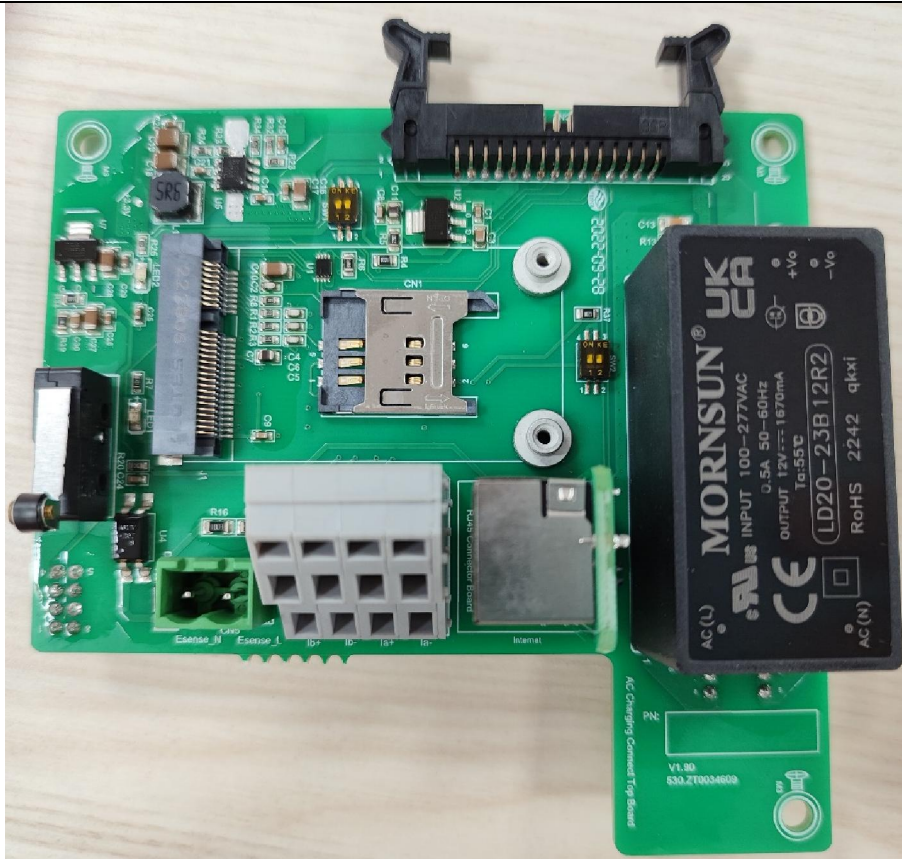
Top view of AC Charging Connect Top Board, V 1.90
