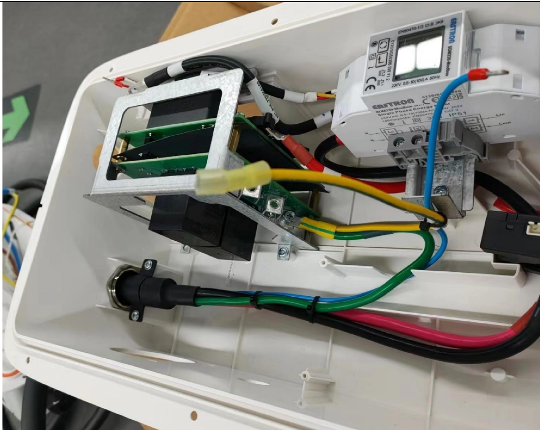
Internal view of the unit
