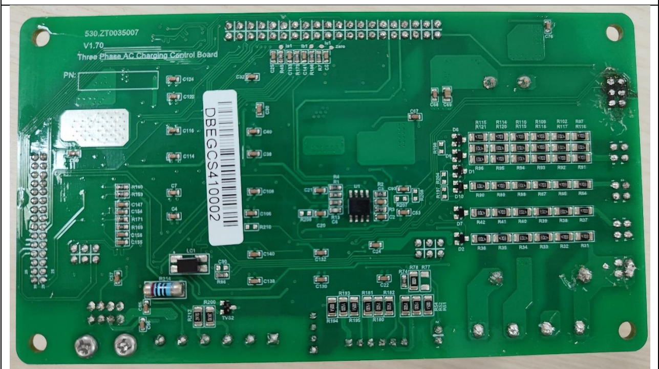
Bottom view of Three Phase AC Charging Control Board, V 1.70
