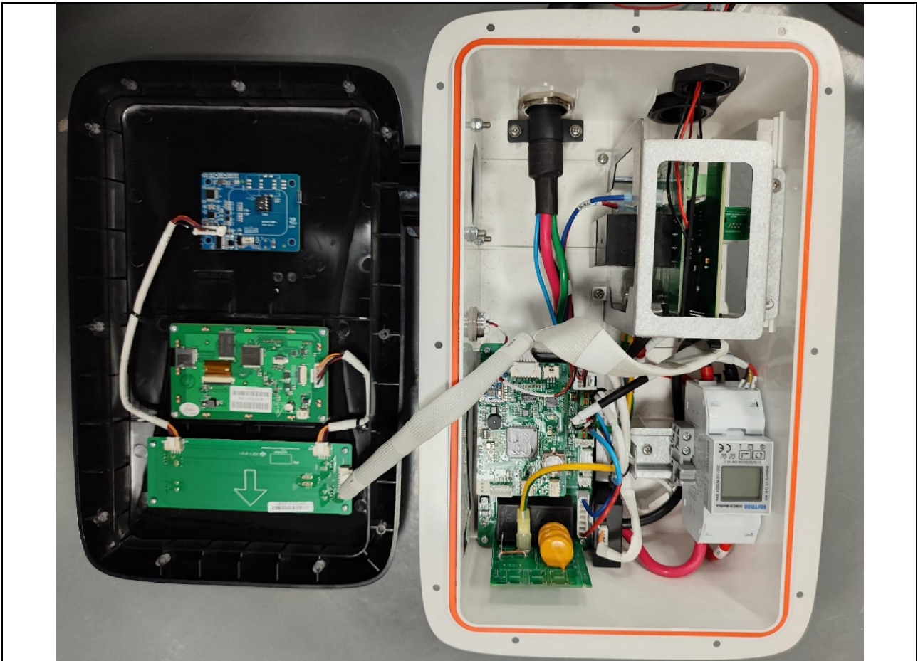
Internal view of the unit. Top cover opened
