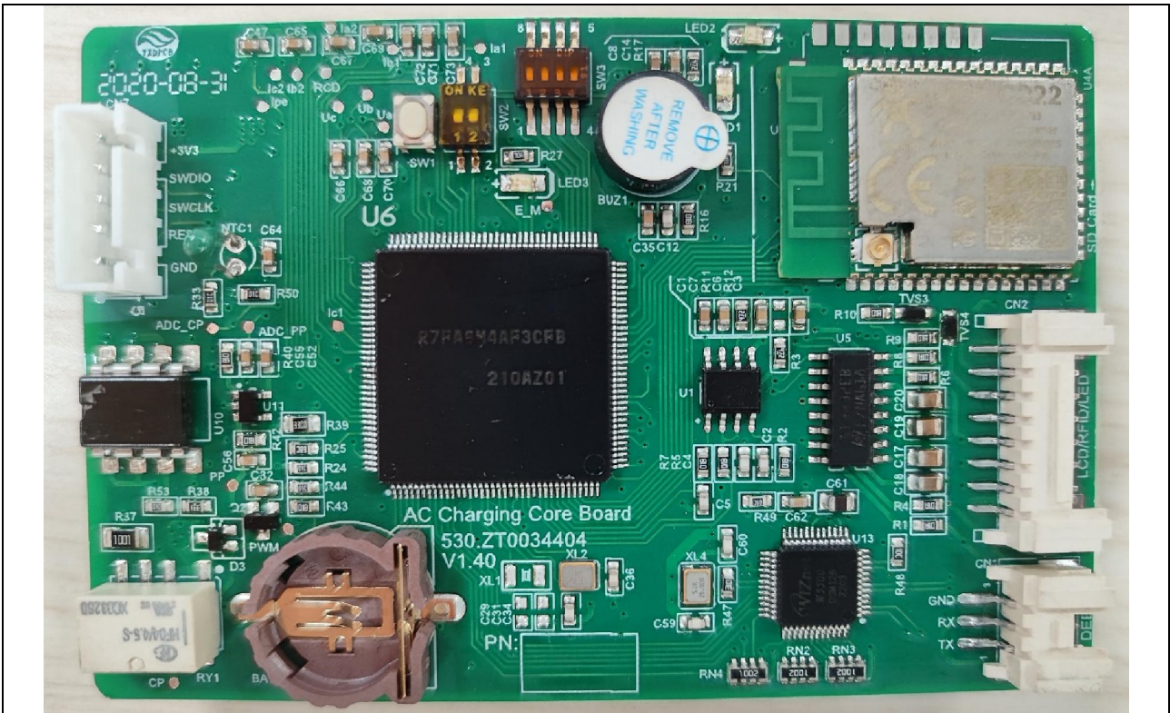
Top view of AC Charging Core Board, V 1.40
