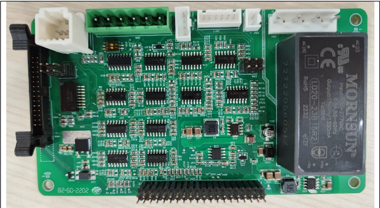
Top view of Three Phase AC Charging Control Board, V 1.70
