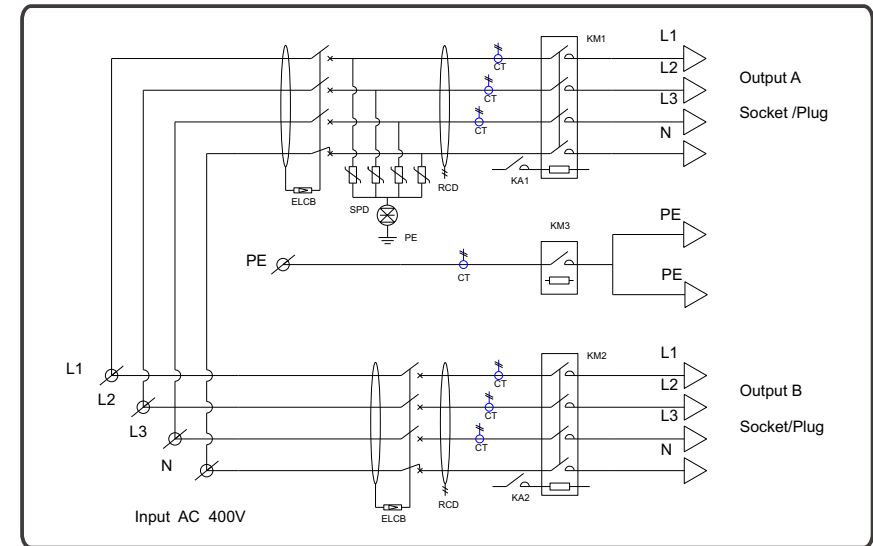
Fig13-1. Main circuit diagram
